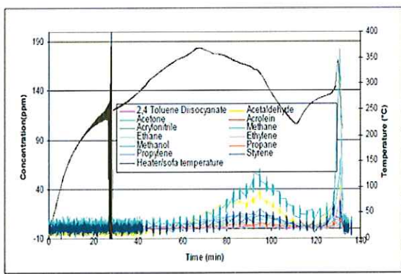
図 26-2 VOC concentrations Versus time at the ceiling
