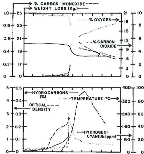
図 26-1 Toxicity of smoke during Chair smoldering tests for Polyurethane foam
