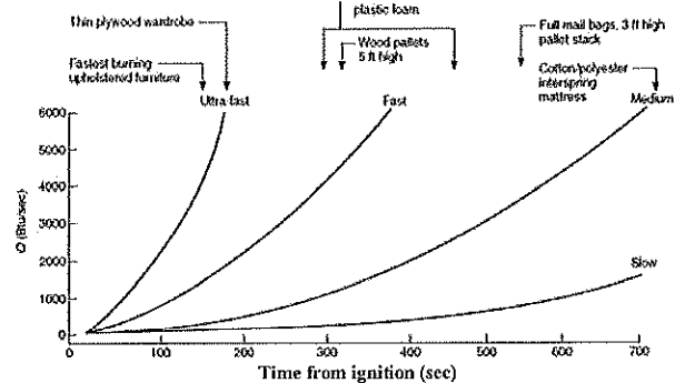
図13-2 Standard Fire Growth Rate Curves. (with some examples of fire test fuels)
