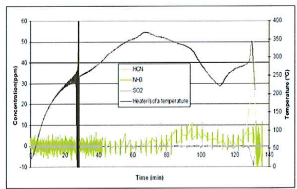
図 26-3 Concentrations of inorganic gases vs time at the ceiling
